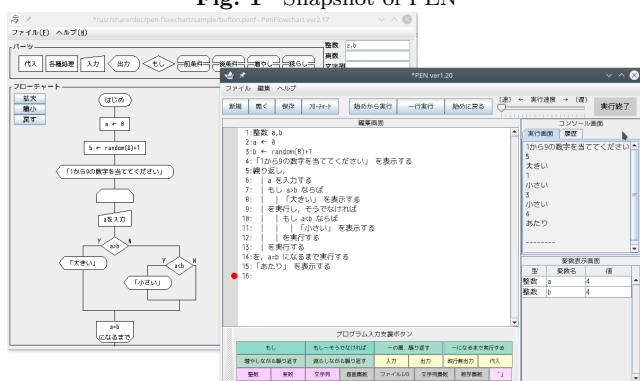
図2 PenFlowchartの実行画面 Fig. 2 Snapshot of PenFlowchart
